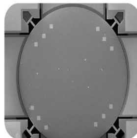
MEMS Mass Sensor
